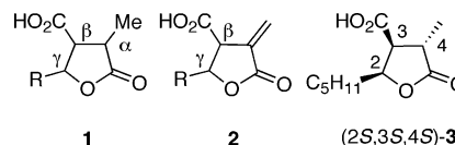
FIGURE 1. Structure of paraconic acids.
